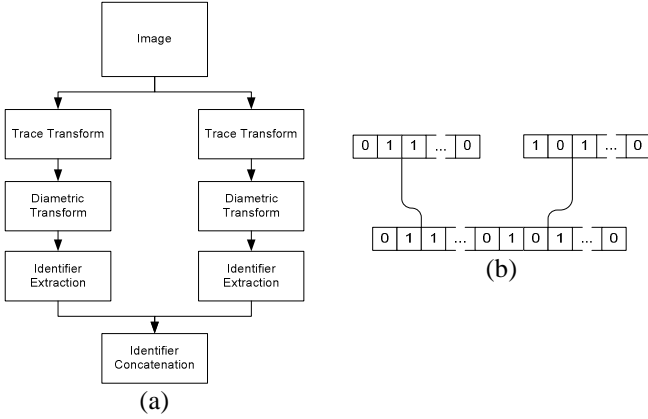
Figure 6. Different combinations of Trace and diametric functionals are used to obtain multiple identifiers (a). Identifiers are then concatenated to form the final image identifier (b).
